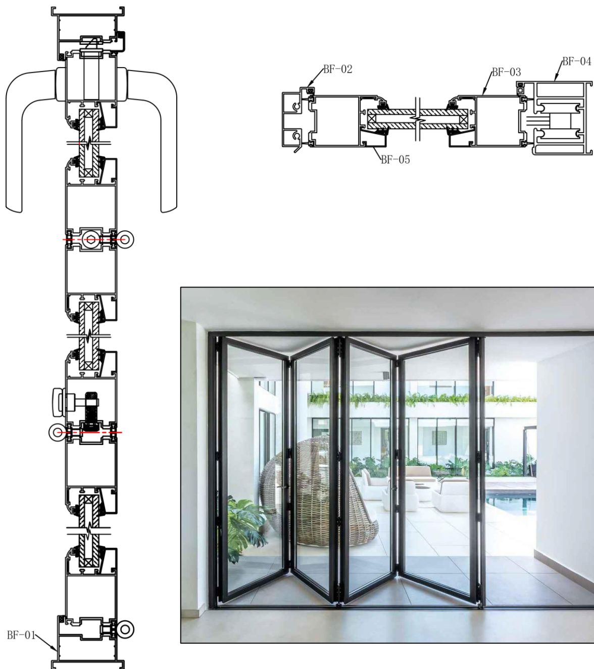
Bifold Doors Concept Drawing
